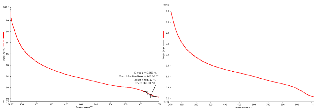
Fig. 2(a) T.G. of ZnO at Temp. 303K
